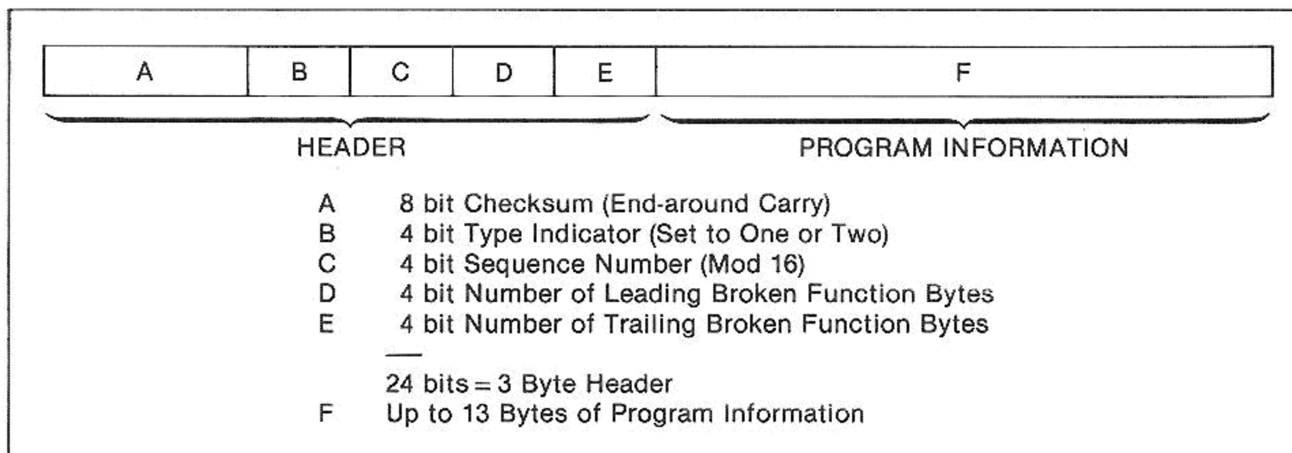
Figure 1. Program Type Bar Code
