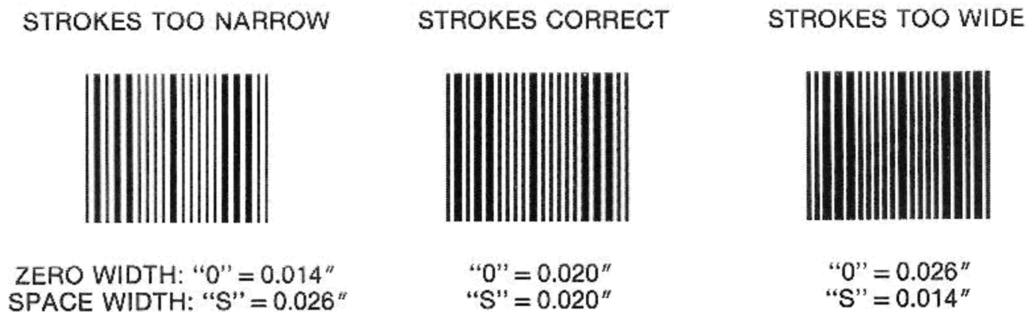
Figure 7. 20-Mil Bar Code Having Excessive Stroke-Width Error
