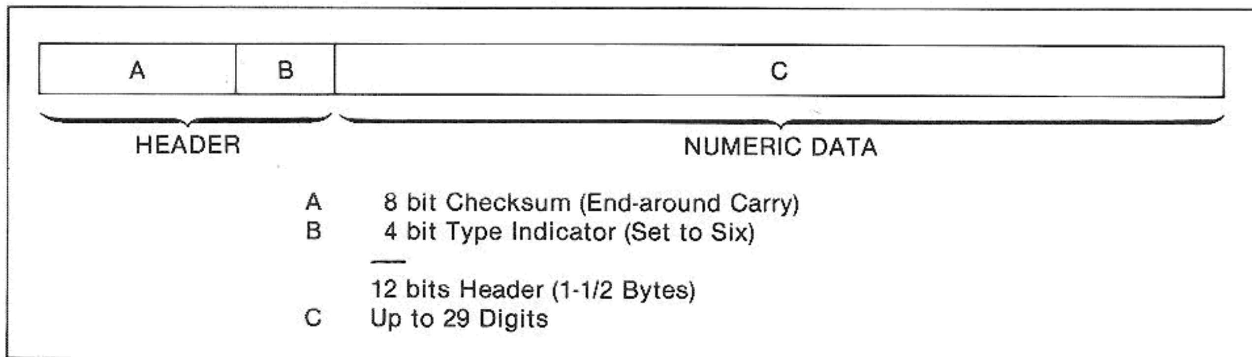
Figure 3. Numeric Data Type Bar Code
