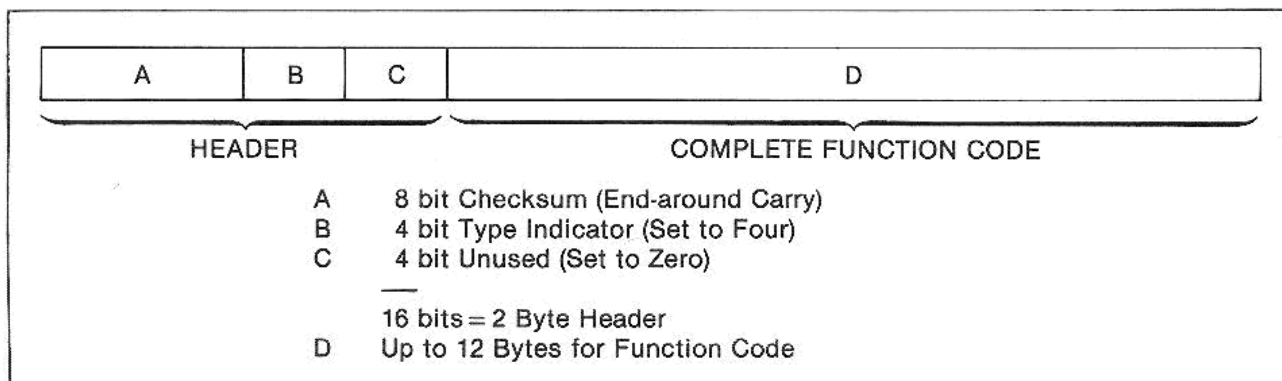
Figure 2. Direct Execution Type Bar Code
