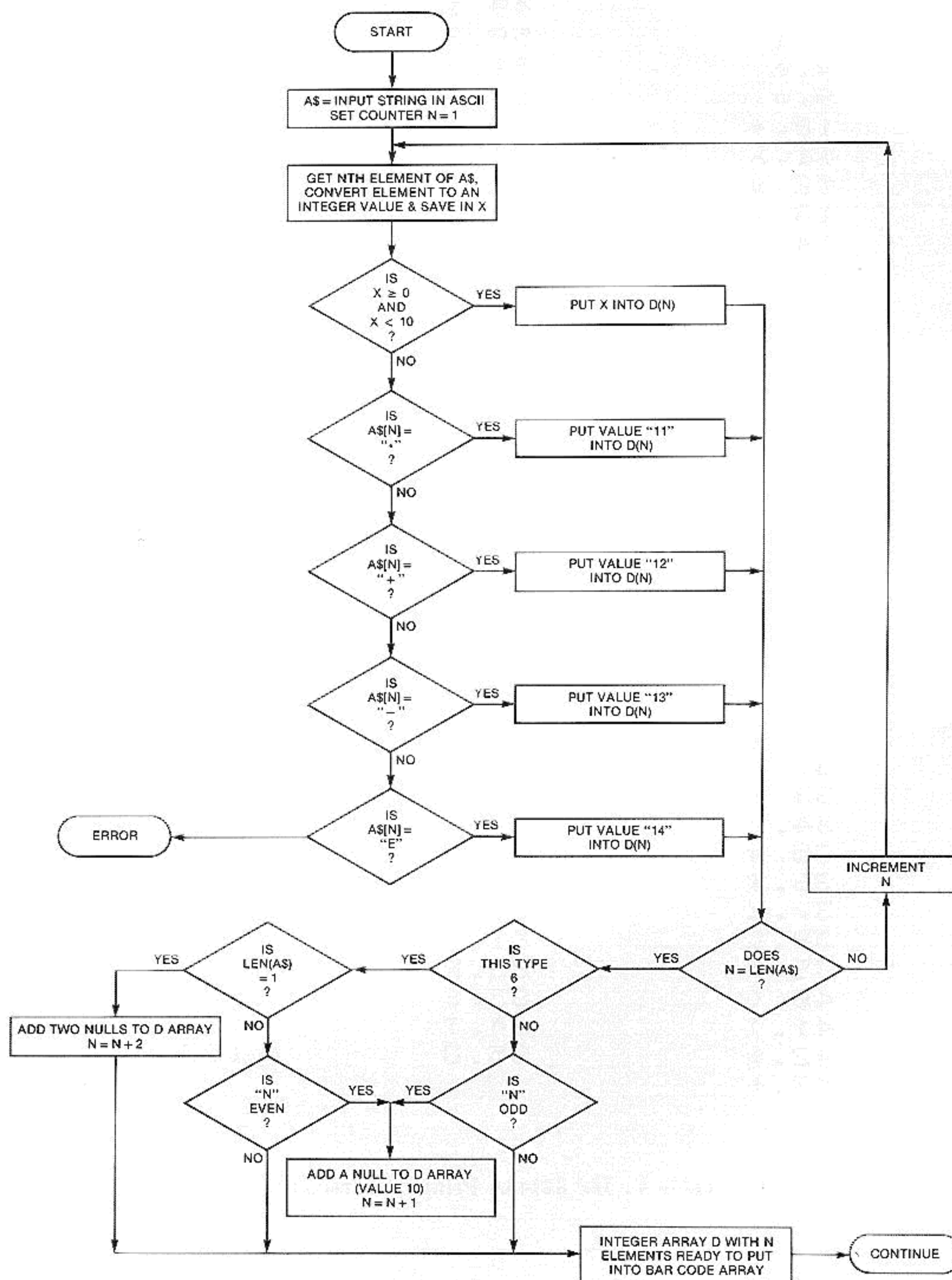
FLOWCHART TO CONVERT ASCII INPUT STRING TO INTERNAL 4-BIT NUMERIC REPRESENTATION
