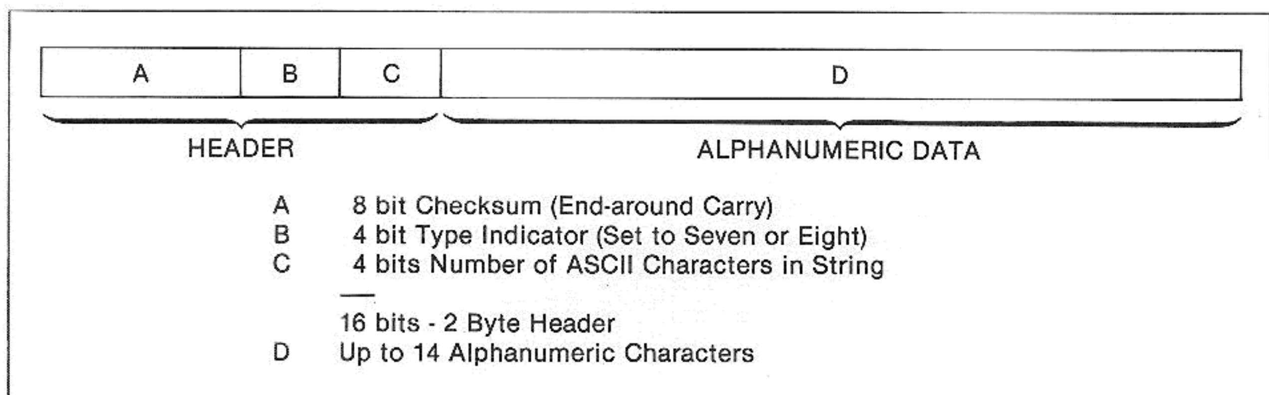
Figure 4. Alpha Data Type Bar Code
